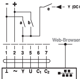
Override control and limiting with DC 24 V with relay contacts (with conventional control or hybrid mode)
