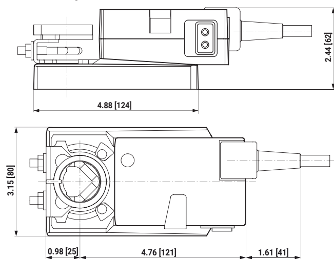
Dimensional drawings NMV-D3-MOD
