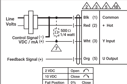
Proportional, CQKB24-SR-RR
