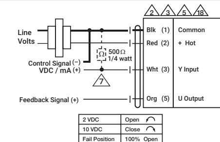
Proportional, CQKB24-SR-LL
