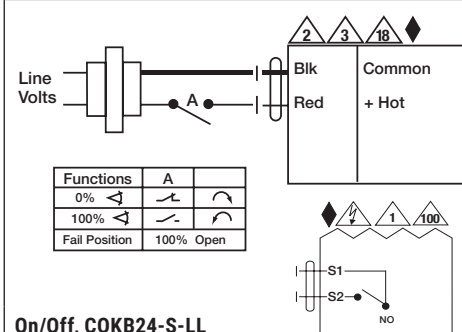
On/Off, CQKB24-S-LL
