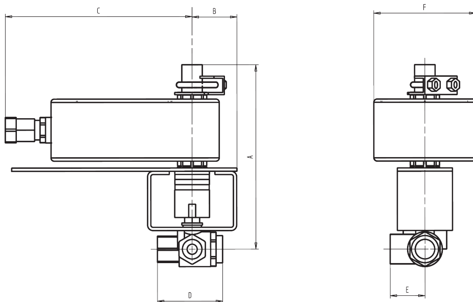
Dimensional drawings
