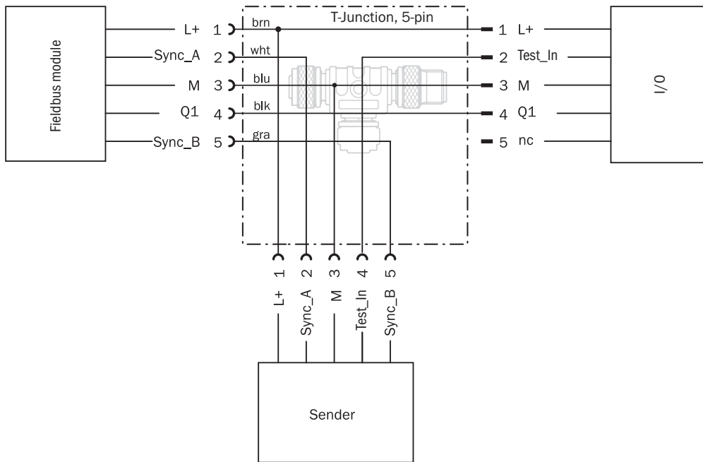
Connection diagram T-junction
