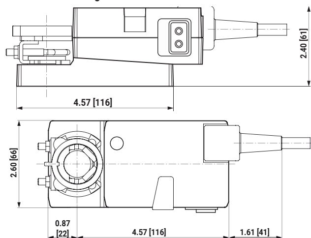
Dimensional drawings LHV-D3-MP
